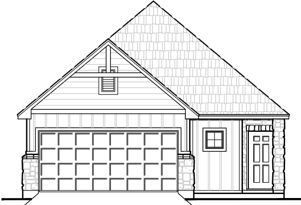
Elevation C
