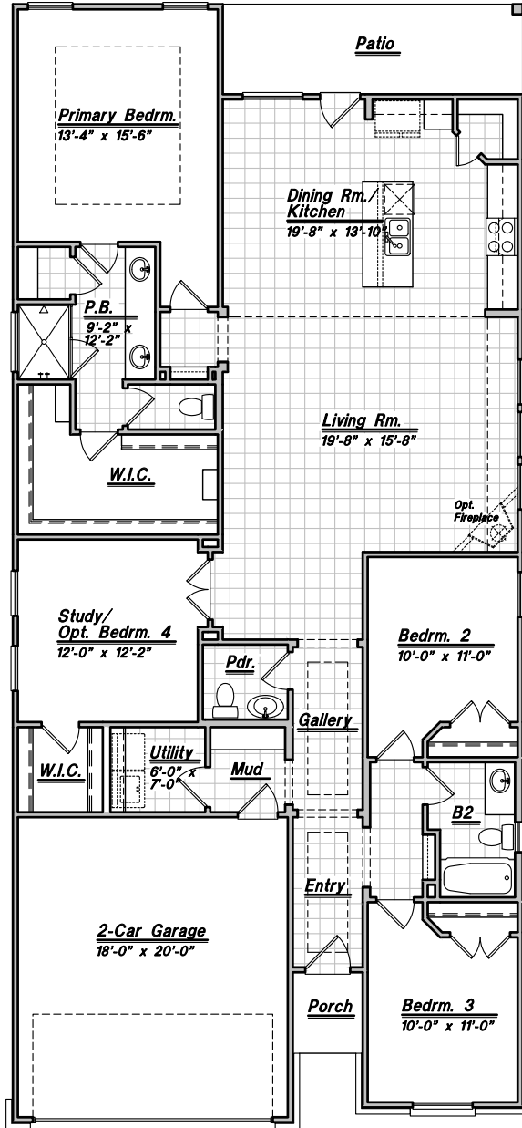
Floor Plan
