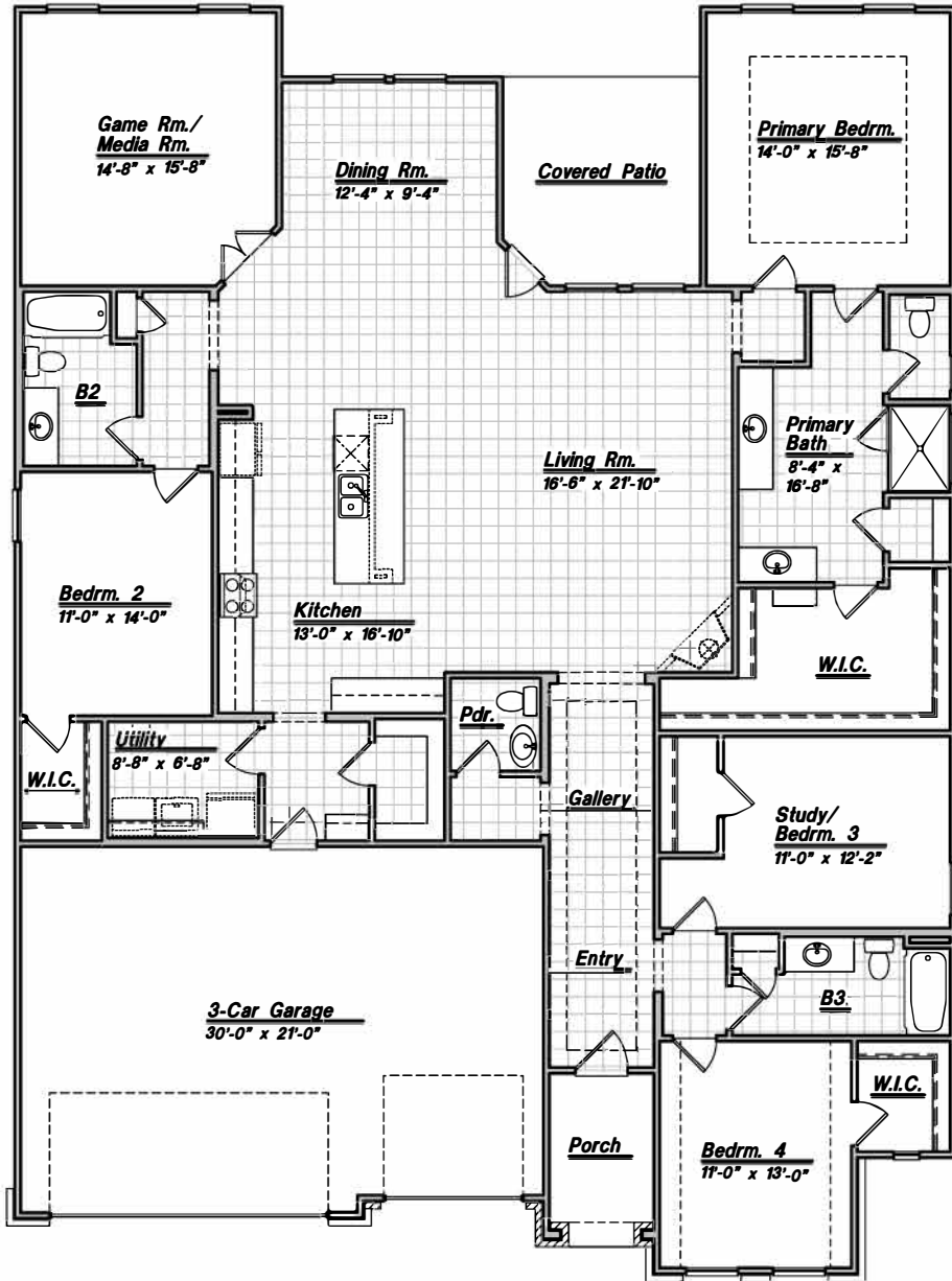
Floor Plan
