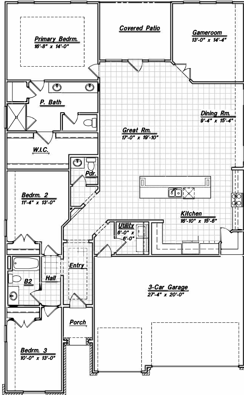
Floor Plan
