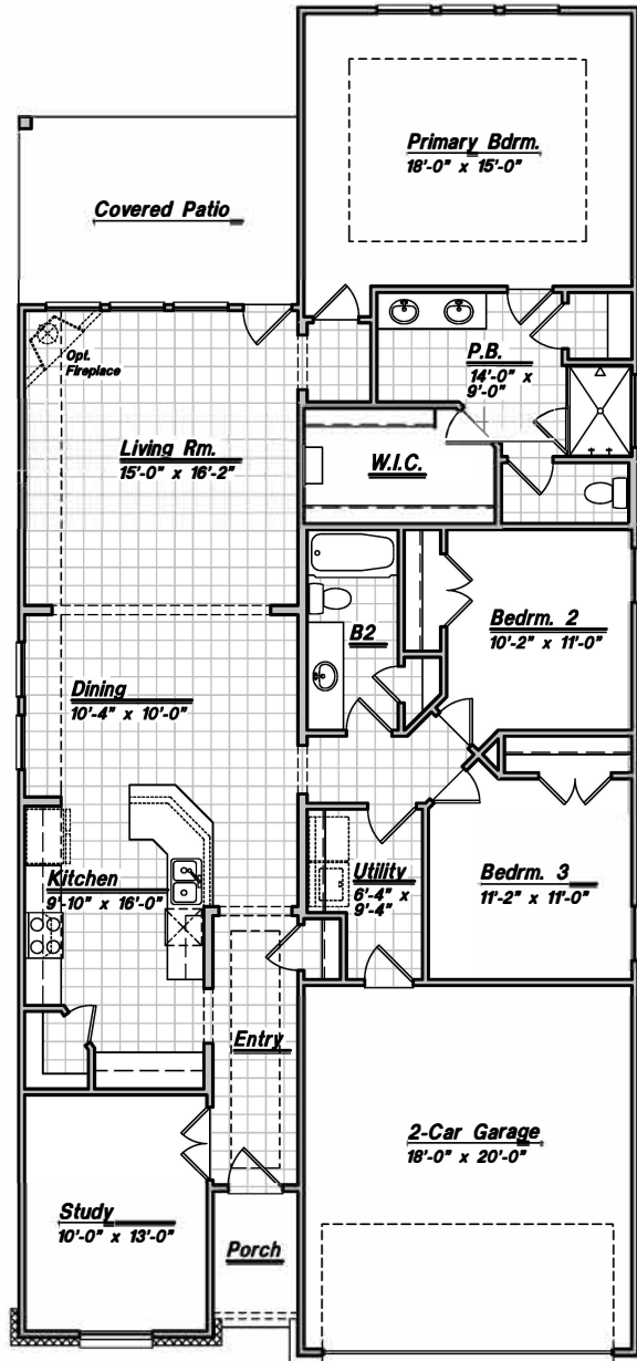
Floor Plan
