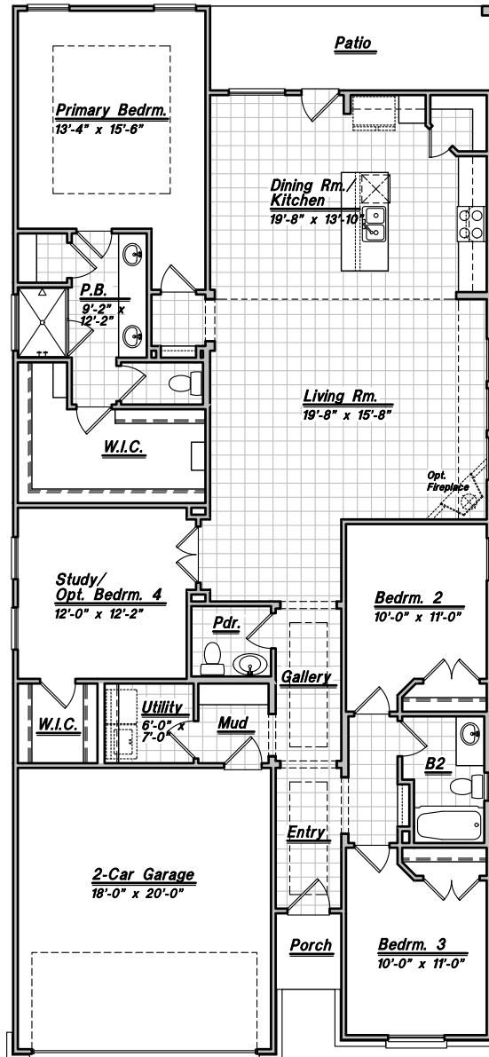
Floor Plan
